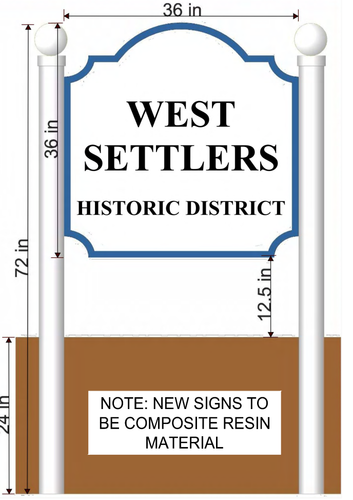
NEW NEIGHBORHOOD SIGN DIMENSIONS DETAIL
